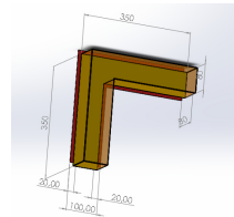
wave 625 L = 90° Winkel
